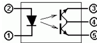
Internal Circuit
